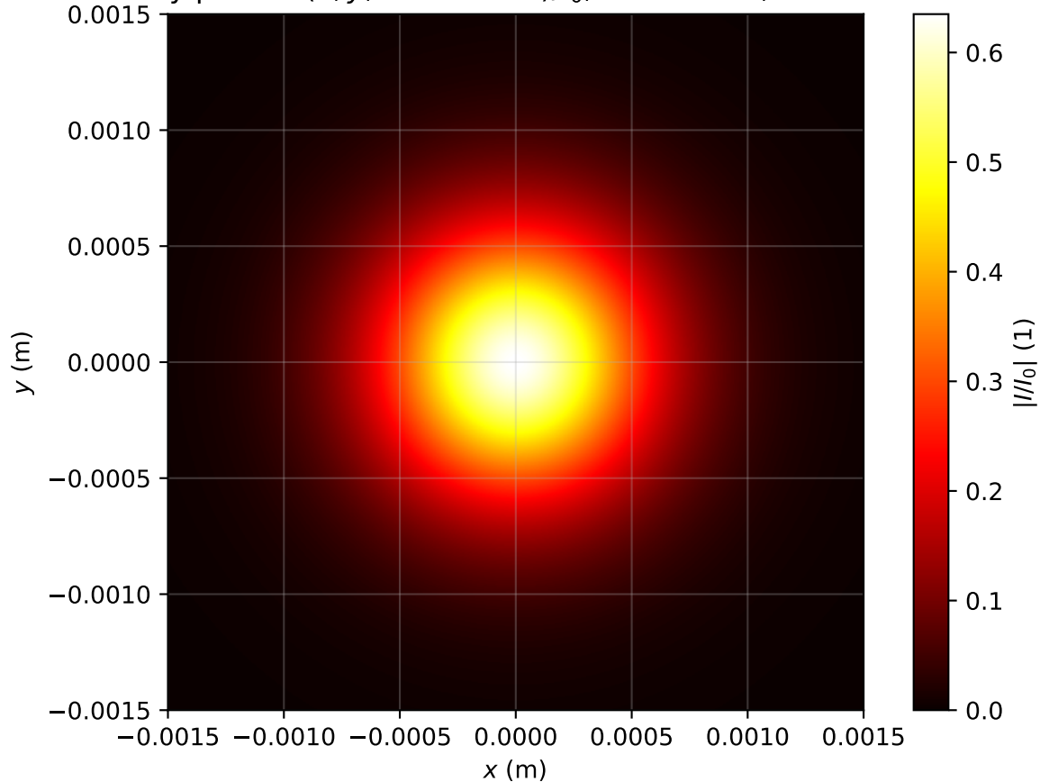
Intensity profile I(x, y, z = 3.184m)/I_0 , P_{in}=0.6P_{cr} , artificial time
